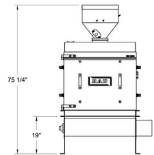
45° UNLOADING HOPPER FOR 6" Ø OR 8" Ø AUGER
